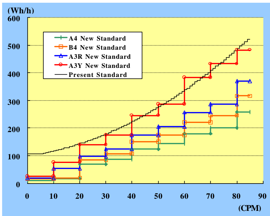
Figure 3: Revised Target Efficiency Values for Photocopiers for 2006, Japan
